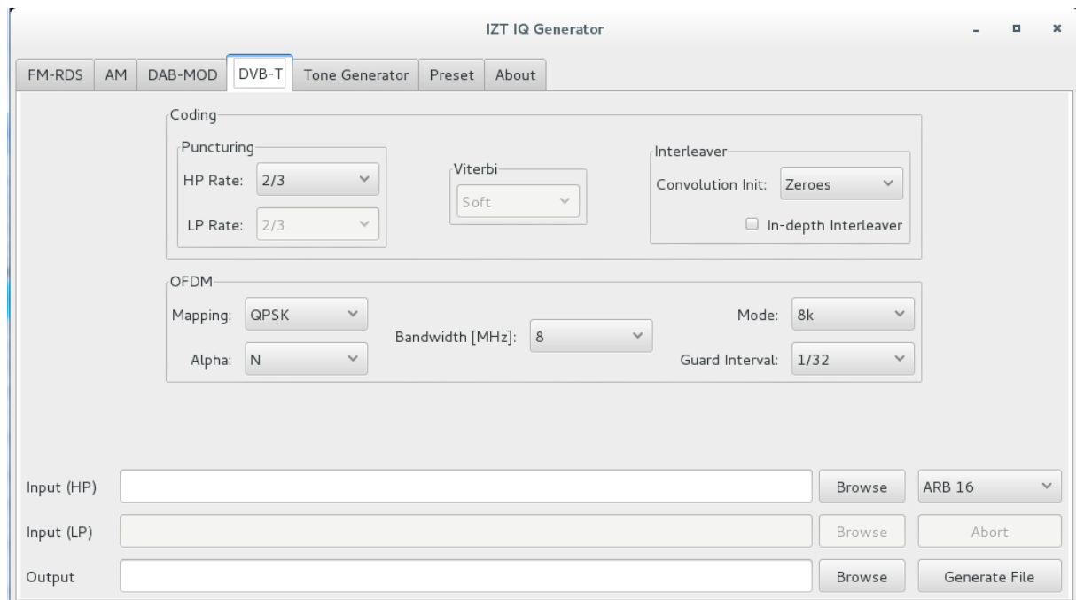
figure 16: Front panel of the IZT DVB-T modulator
