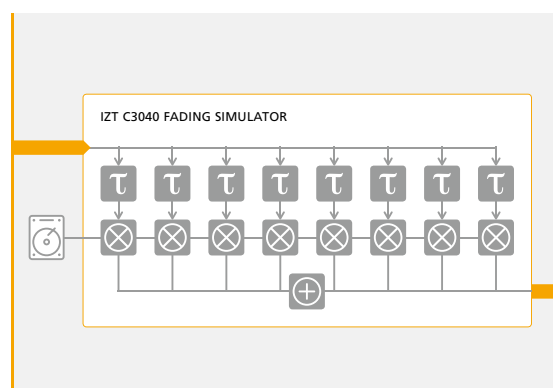
FIGURE 15: BLOCKDIAGRAM OF THE FADING SIMULATOR
