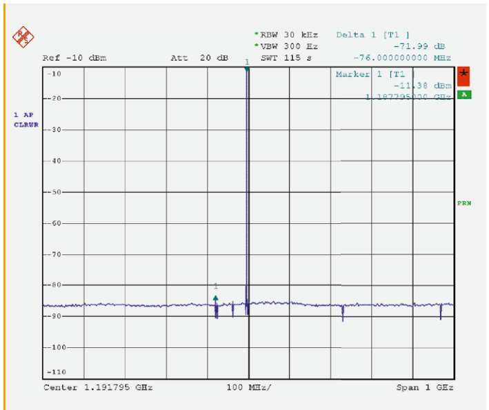
FIGURE 16: EXCELLENT SPURIOUS PERFORMANCE AND SIGNAL-TO-NOISE RATIO
