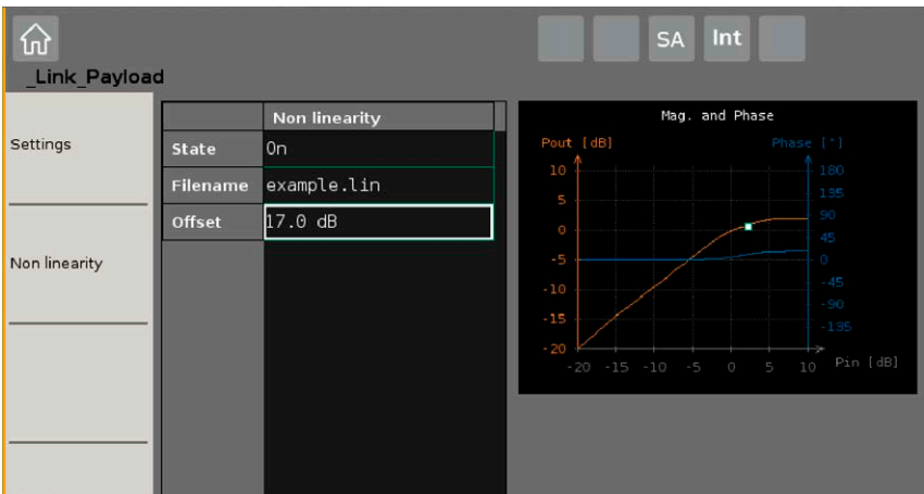
FIGURE 4: NONLINEARITY CONTROL
