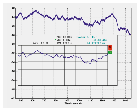
FIGURE 13: EXAMPLE OF A RAIN FADE SIMULATION
