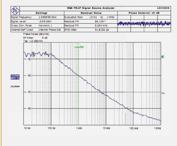
FIGURE 9: SIMULATED PHASE NOISE “DVB-S2 TYPICAL”
