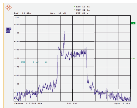
FIGURE 14: RICIAN FADING
