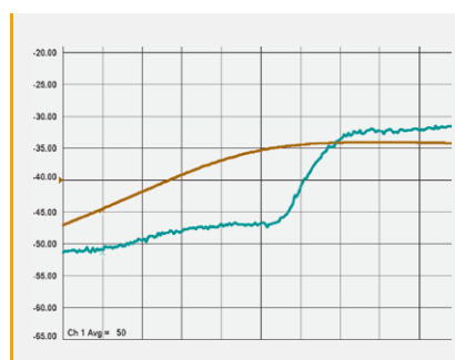
FIGURE 10: EMULATION OF PAYLOAD NONLINEARITY
